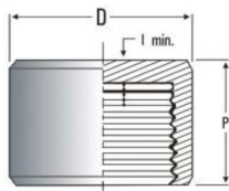
Dilimli KEK THREADED CAP
