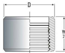
Dilimli YARIM MANILON THREADED HALF COUPLING
